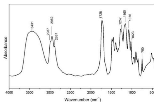
Figure 3. FTIR spectrum of pHEMA.
