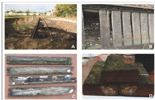
Fig. 2. Detail of locomotive turntable status: A - Structure consists in wooden slats of Schinopsis sp. within metal framework; B - slats in advanced status of deterioration caused by environmental and biological factors; C - Samples acquired for simulating the same degradation status than wooden turntable in laboratory; D - Detail of wood decay fungi found and its biodegradation (inside view).
