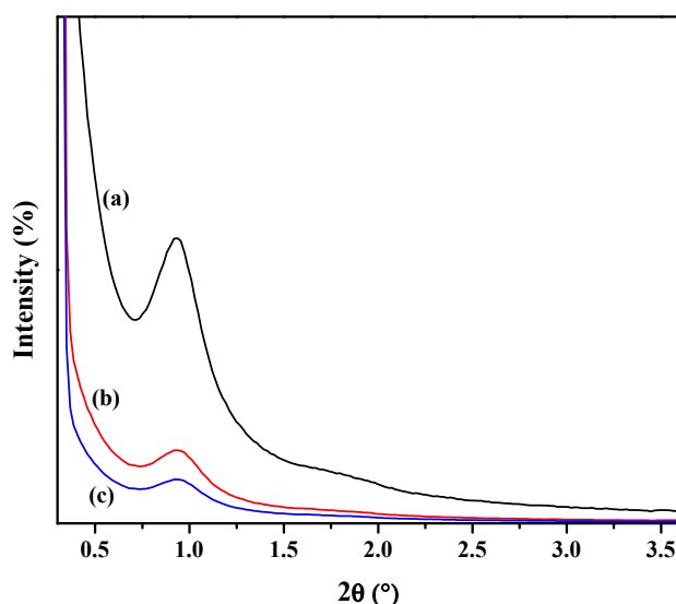
Figure 1. Small angle X-ray scattering patterns of (a) MA, (b) BiVA-MA, (c) BiEG-MA.
