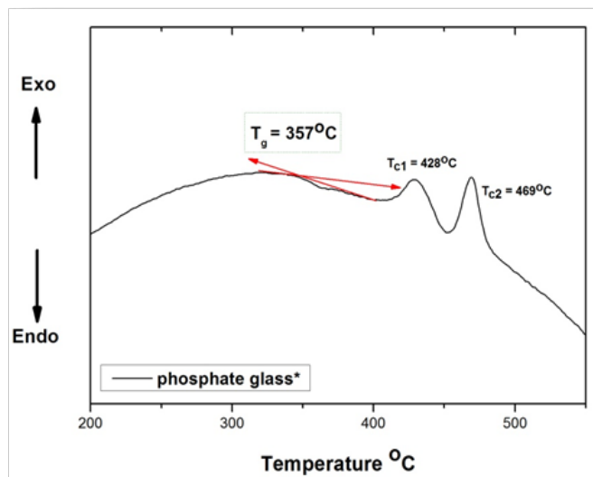
Figure 3 [LBPB4] DTA heating curve.
