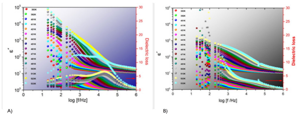
Figure 4 Real part of the complex permittivity of: A) NF-LBPB4 pristine composite and B) NF-LBPB4 treated 1 h at 703K.
