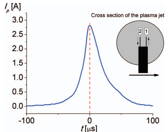
FIG. 4. Average I_p waveform for V = -31 \text{ V} . The probe location corresponding to the maximum of I_p (indicated by the vertical dotted line) is shown in the inset.
