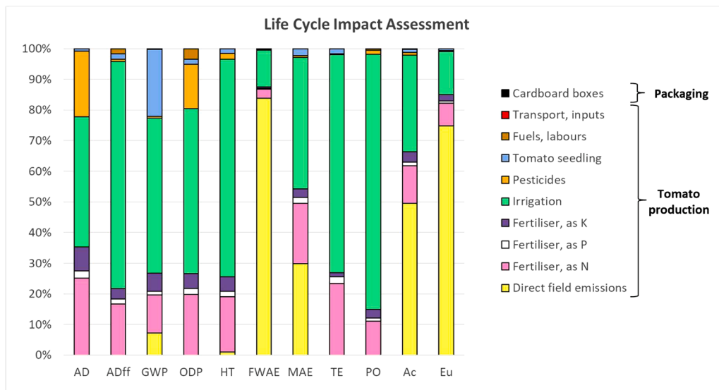
Fig. 2. Process contribution to impact categories for tomato production in Mendoza, Argentina.
