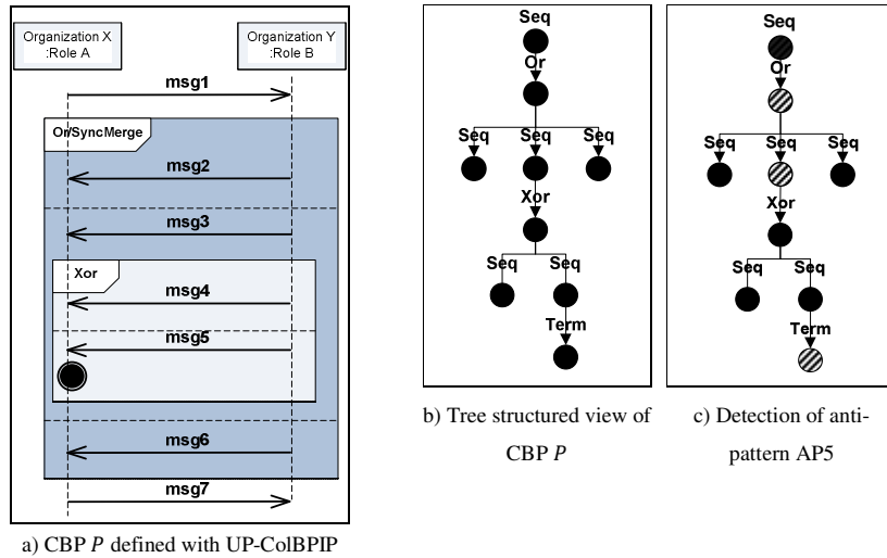
Fig. 5. Example of Anti-Pattern AP5
