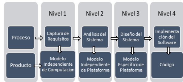
Figura 1. Model-Driven Architecture
