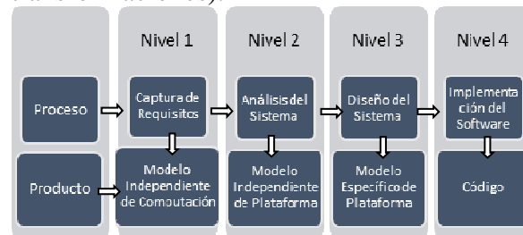
Figura 1. Model-Driven Architecture
